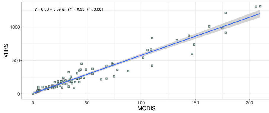
Figure S4: Scatter plot of the number of fire points per month sensed by MODIS and VIIRS sensors for the period 2012-2018
