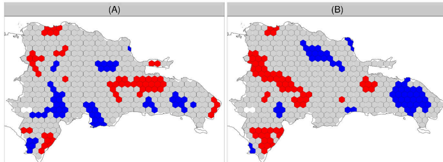
Figure 5: LISA maps (local indicators of spatial association maps) of (A) forest loss per unit area averaged per year for the period 2001-2018, and (B) fire points per km 2 averaged per year within forest cover for the same periods using the MODIS dataset. The Tukey's Ladder of Powers transformed versions of the variables were used as inputs in all cases. Each hexagon was classified either as HH cluster—group of cells in which high values are surrounded by other high values—(depicted in red) , LL cluster—cells with low values surrounded by other low values—(depicted in blue) , or no significant spatial association (grey) regarding the corresponding variable.
