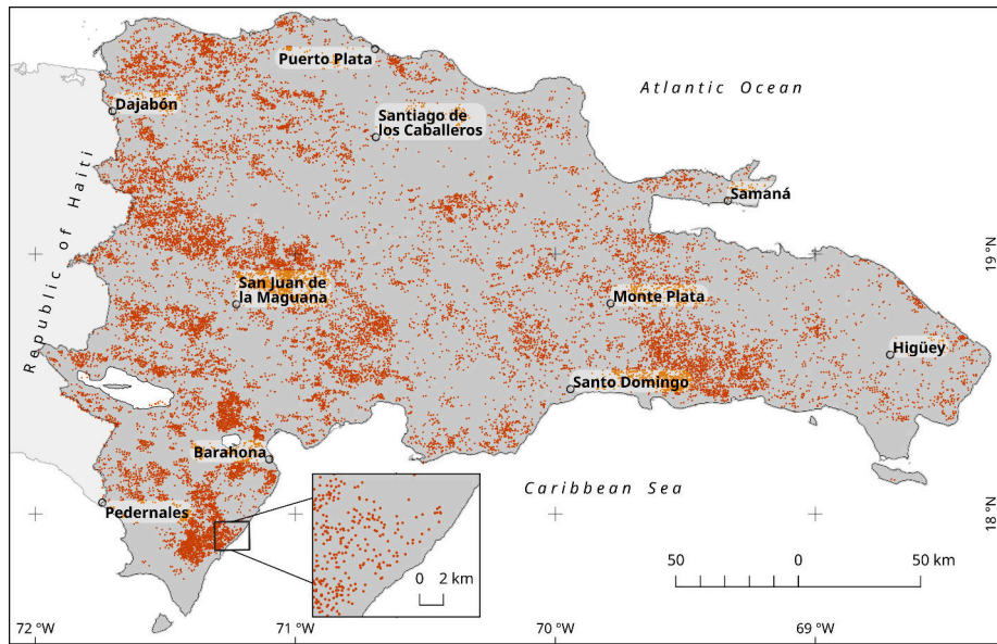
Figure S1: MODIS fire points/hotspots from 2001 to 2018 for the DR mainland. This is a noise-free version of the original dataset, which excludes unrelated fire points (e.g., burning landfills and industrial furnaces). See text for details.
