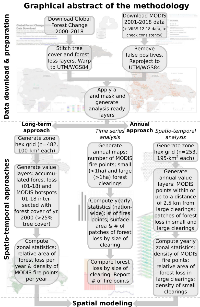
Figure 2: Graphical abstract of the methodology. See text for details and see the Data and code availability section for provided scripts.
