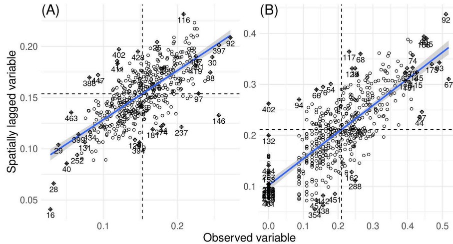
Figure S5: Moran scatterplots of the transformed versions of the analyzed variables. (A) Average forest loss per unit area per year of the period 2001-2018. (B) average number of fire points per \text{km}^2 per year in the period 2001-2018 using MODIS dataset.
