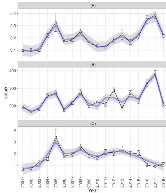
Figure 7: Yearly averages per 100 km 2 of (A) Forest loss area (in km 2 ) of large clearings (>1 ha in size); (B) Number of small clearings (<1 ha in size); (C) Number of fire points remotely sensed by the MODIS sensor in or around forest loss patches
