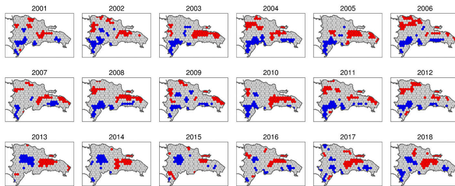
Figure 10: Yearly LISA maps (local indicators of spatial association maps) of transformed forest loss density data of small clearings. Same legend as in Fig See Figure 9 for colour legend of hexagons.
