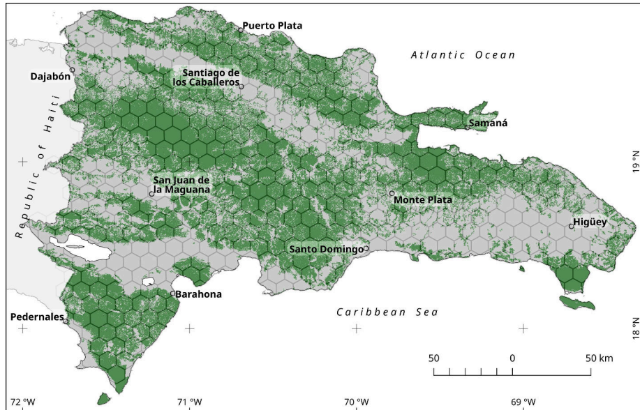
Figure 3: DR forest cover in the year 2000. Areas with a canopy closure equal to or greater than 25% in tree cover map of Hansen et al. (2013) were classified as forest. The hexagonal grid overlaid was used for zonal statistics computations of the long-term approach. See text for details.
