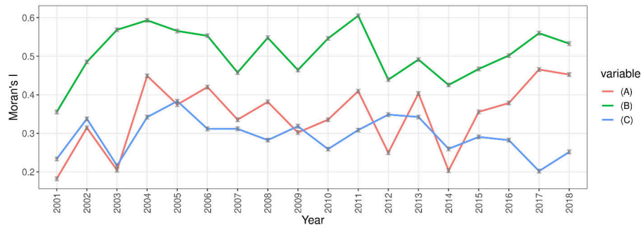
Figure 8: Moran's I (used to assess spatial autocorrelation) evolution from 2001 to 2018 for the transformed versions of yearly averages per 100 km 2 of: (A) Forest loss area of large clearings (>1 ha in size); (B) Number of small clearings (<1 ha in size); (C) Number of fire points located inside or around forest loss patches recorded by the MODIS sensor
