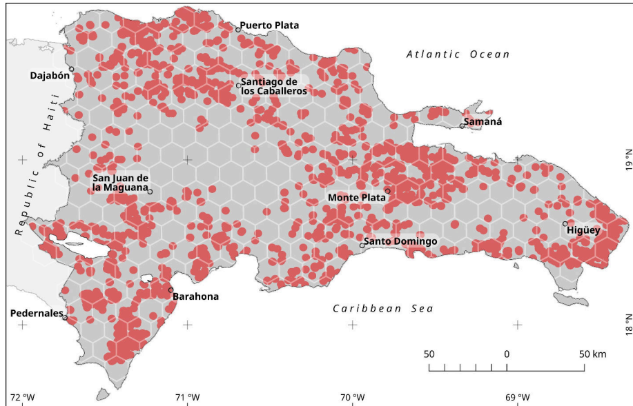
Figure S6: Example of the 2013 forest loss areas and their vicinity (red shaded areas) used in the annual trend approach. These areas were generated by adding a buffer zone of 2.5 km around each patch larger than 1 ha in area from the loss year dataset (Hansen et al., 2013). The hexagonal grid, depicted as an overlay, was used for zonal statistics computations. See text for details.
