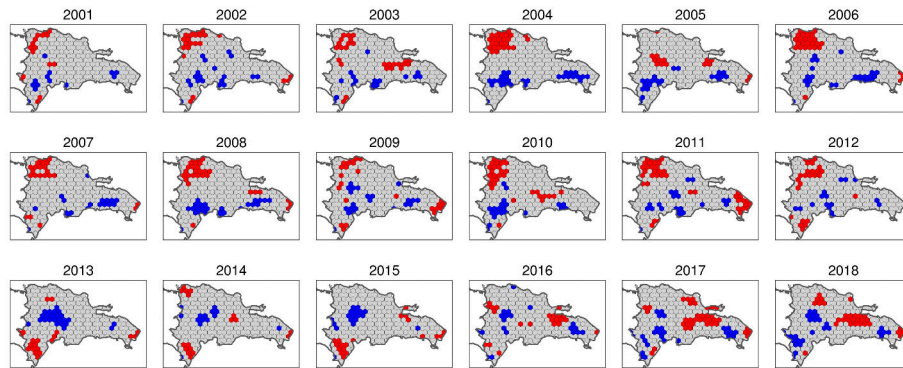
Figure 9: Yearly LISA maps (local indicators of spatial association maps) of transformed forest loss density data of large clearings. Red represents HH clusters, blue depicts LL clusters, and grey shows no significant spatial association.
