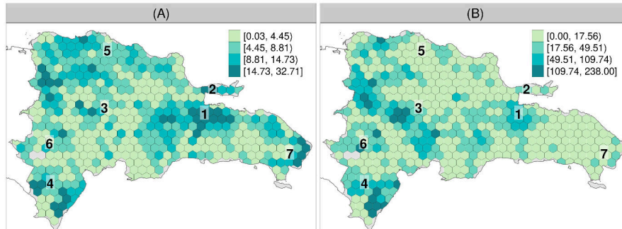
Figure 4: (A) Forest loss (in \text{km}^2 per 100 \text{ km}^2 ) for the period 2001-2018. (B) Number of fire points per 100 \text{ km}^2 within forest cover for the period 2001-2018 using MODIS dataset. The baseline year for forest cover is 2000. Reference locations: 1 Los Haitises; 2 Samaná Peninsula; 3 Cordillera Central mountain range; 4 Sierra de Bahoruco; 5 Cordillera Septentrional; 6 Sierra de Neyba; 7 Eastern Region.
