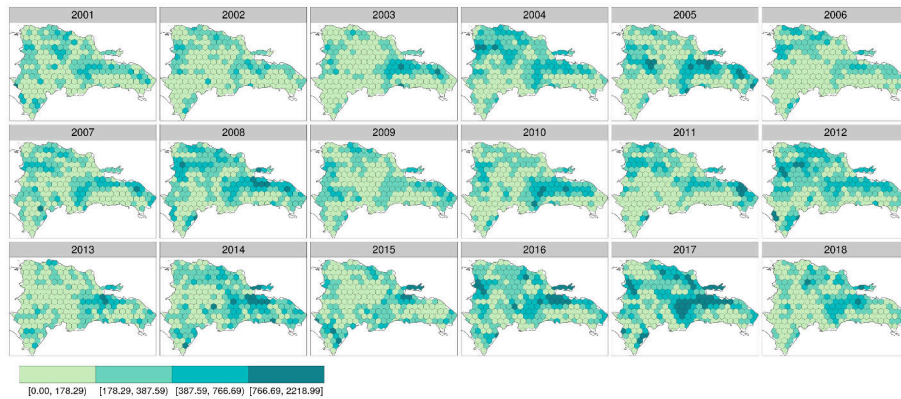
Figure S9: Yearly number of forest loss patches smaller than 1 ha (in km 2 per 100 km 2 ) for the period 2001-2018
