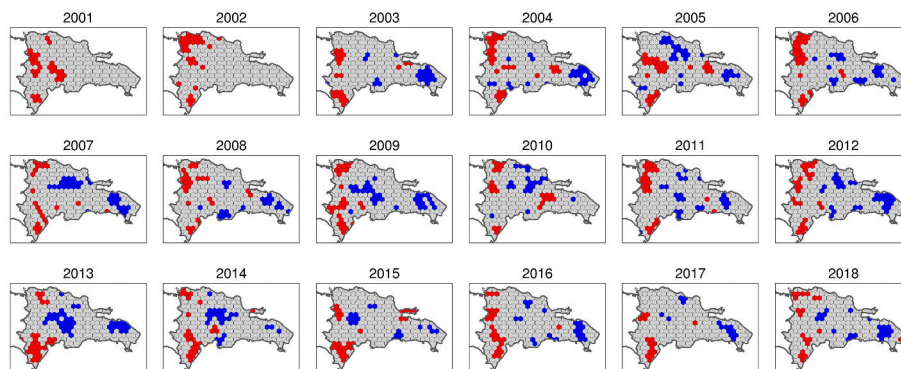
Figure 11: Yearly LISA maps (local indicators of spatial association maps) of transformed MODIS fire density data. Same legend as in FigSee Figure 9 for colour legend of hexagons.
